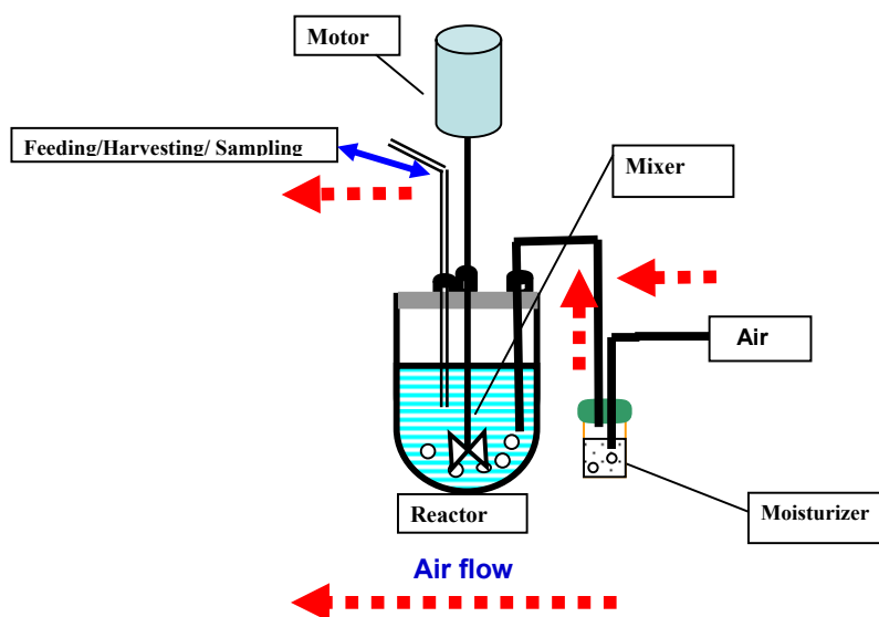
Figure 1. Experimental apparatus using 3 liter vessel (inoculum maintenance)
