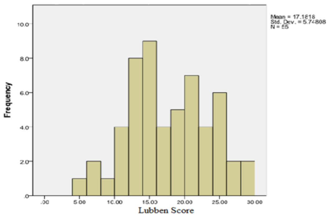
Figure 4. Histogram of Lubben Score for Non-Married Participants
