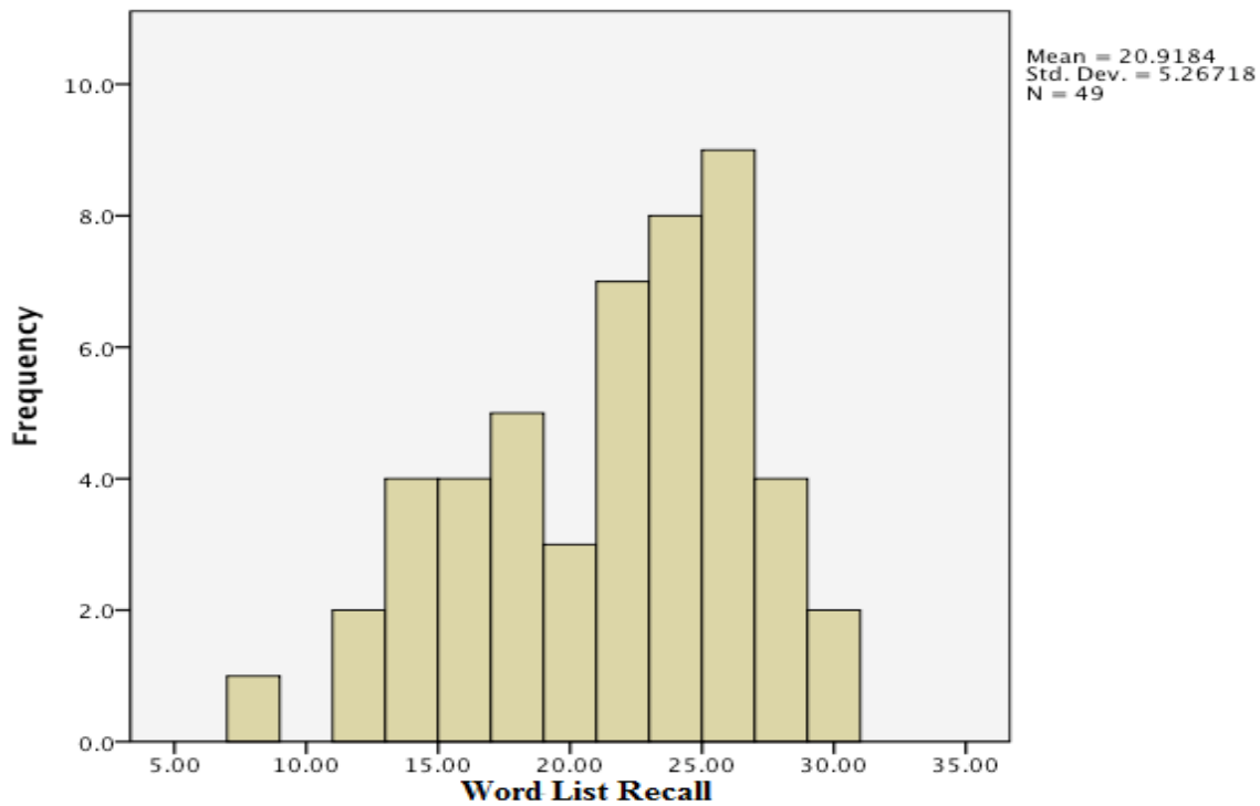
Figure 1. Histogram of Word List Recall for Married Participants
