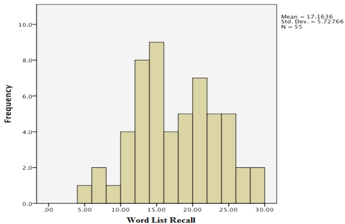
Figure 2. Histogram of Word List Recall for Non-Married Participants
