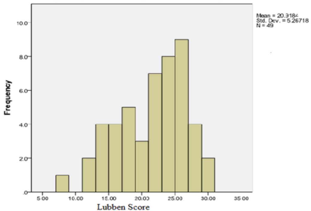
Figure 3. Histogram of Lubben Score for Married Participants
