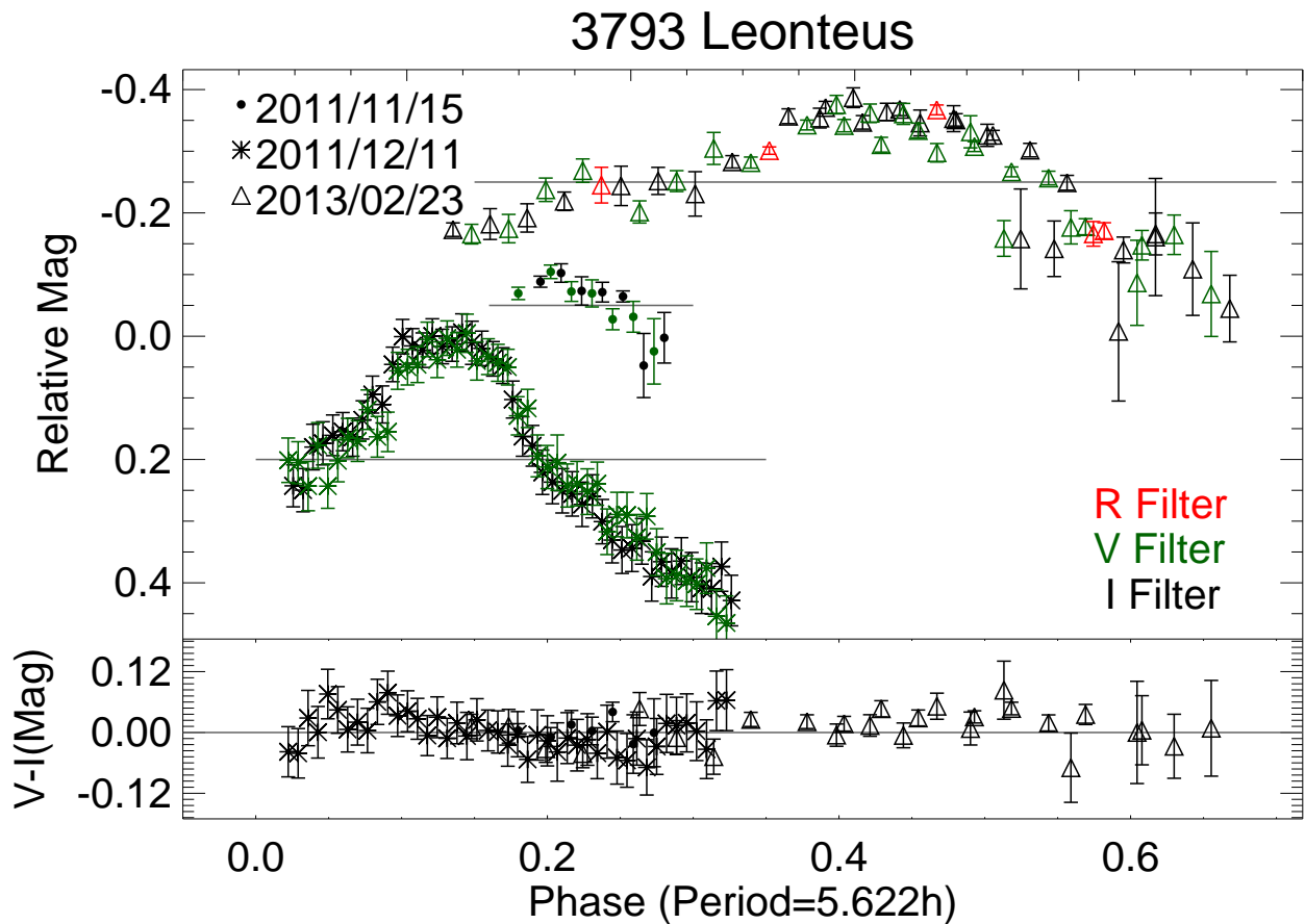
Figure 3.17: Light curve (top) and V - I color curve (bottom) for (3793) Leonteus during 2011 and 2013. Due to the large variation in light curve shape and amplitude, individual datasets have been offset from one another.
