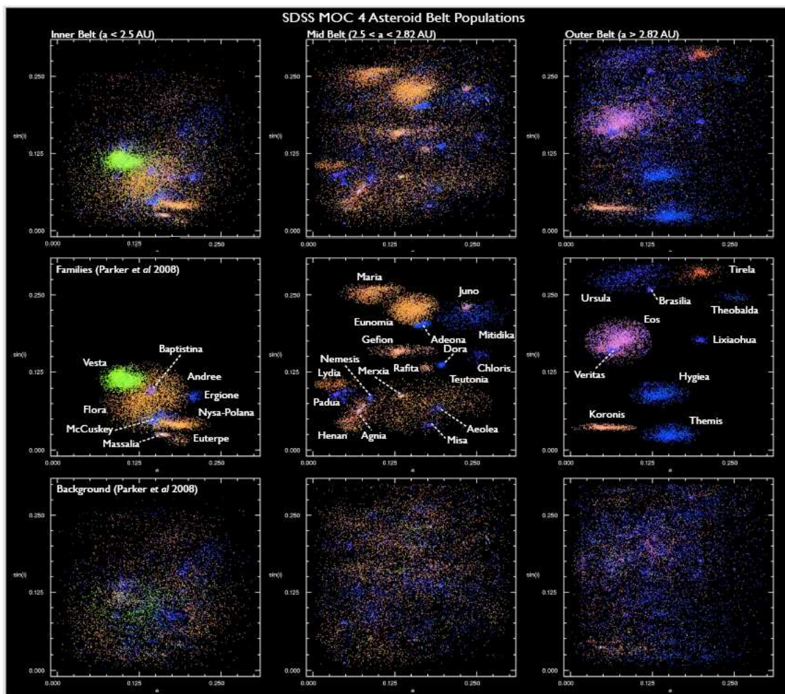
Figure 1.2: Figure from described by Parker et al. (2008) a . Sloan Digital Sky Survey Moving Object Catalog 4 data for Main Belt Asteroids. Each plot shows eccentricity vs. sine of the inclination for objects in the Inner Main Belt ( a < 2.5 AU, left), Middle Main Belt ( 2.5 \text{ AU} < a < 2.82 AU, center), and Outer Main Belt ( 2.82 \text{ AU} < a < 3.5 AU, right). The top row is all of the MOC4 data colored by the principal component a^* , the middle row is only families, and the bottom row is background objects with collisional families removed.
