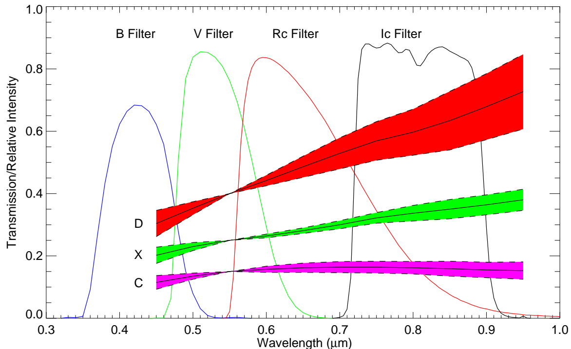
Figure 2.7: Three standard spectra of the Bus-DeMeo taxonomy presented in DeMeo et al. (2009) . The standard spectra are normalized at 0.55\mu\text{m} and offset from each other by an arbitrary amount. The variation in possible spectra that should be considered within each taxonomic group is depicted via the 1\sigma range shown as a solid colored region associated with each taxonomy. The three spectra shown here were chosen as representative of the Jupiter Greeks and Trojans because numerous surveys (e.g. DeMeo & Carry 2013 ) have failed to find evidence of other types within the camps. The spectra are restricted to the visible range and overlaid above the transmission curves for the BVRI filters used for this project (specifically as reported for the 1.0-m). The relative slopes and variations of these standard spectra allow us to calculate the regions in color space where such objects would appear.
