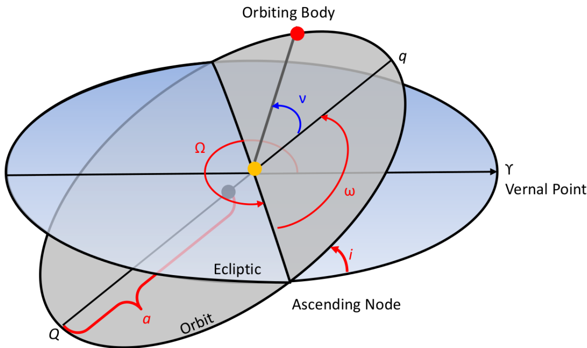
Figure A.1: A graphical depiction of the angular orbital elements described in this section.
