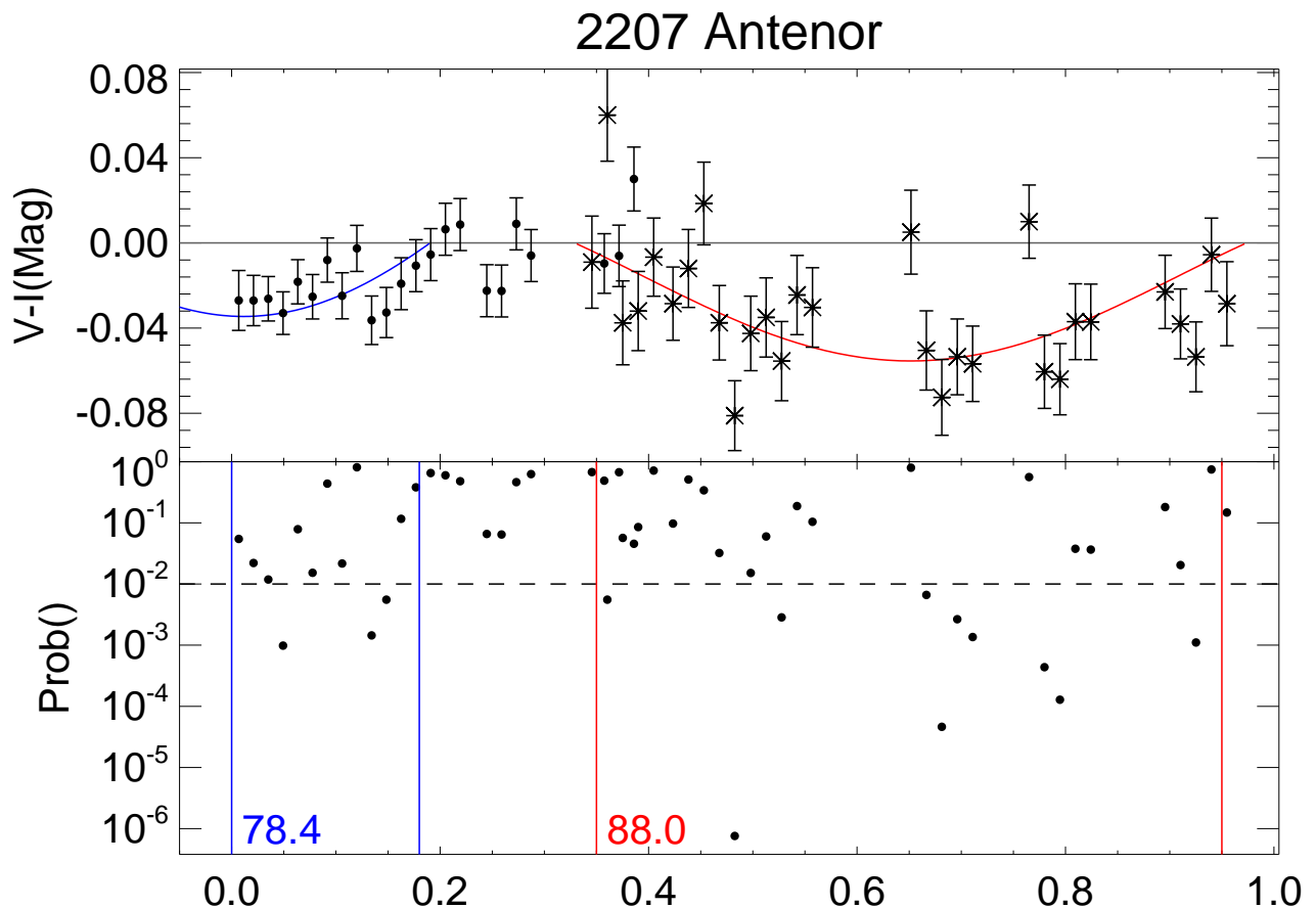
Figure 3.8: Color curve (top) and Individual Probability curve (bottom) for (2207) Antenor during November 2011 and September 2012. We model two potential features (as described in Subsection 3.3.2 ) centered at phase 0.0 and 0.65 with a confidence level of 78.4% and 88.0% respectively. However, due to the time between these two epochs and the lack of a highly precise period, these features could possibly be the same feature, partially sampled on two different dates. The dashed line shows a 99% probability that a data point represents color change. The symbols used in the color curve are the same as those used in Figure 3.7 .
