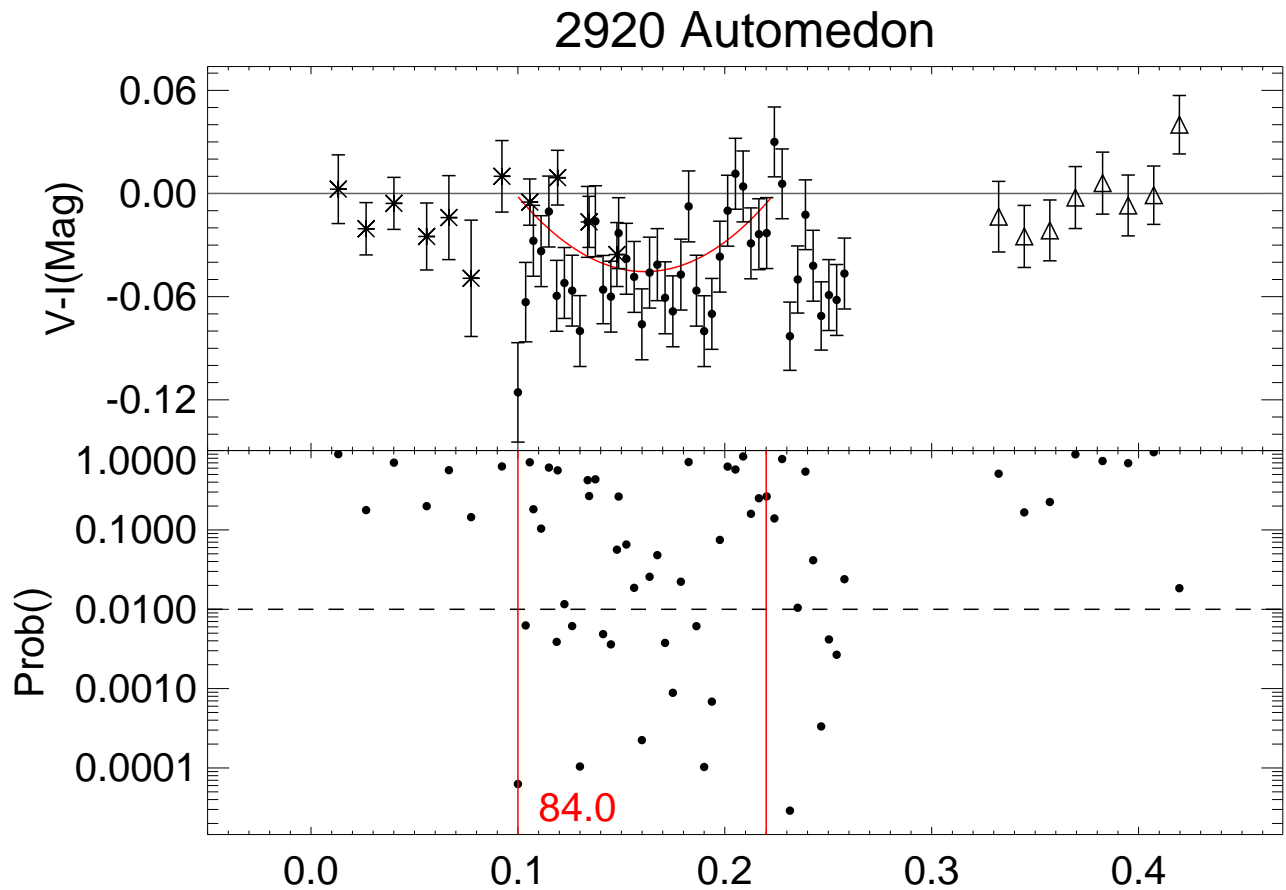
Figure 3.12: Color curve (top) and Individual Probability curve (bottom) for (2920) Automedon during December 2011 and February 2013. We model one potential feature (as described in Subsection 3.3.2 ) centered at phase 0.16 with a confidence level of 84.0%. The dashed line shows a 99% probability that a data point represents color change. The symbols used in the color curve are the same as those used in Figure 3.11 .
