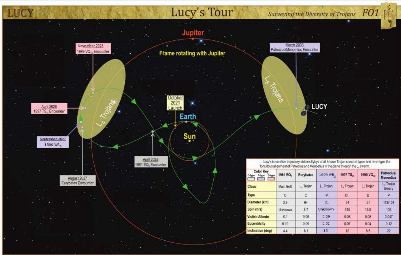
Figure 6.1: Figure credit: Levison & Lucy Science Team (2016) . A full figure description can be found in the original source. The spacecraft is scheduled to visit members of every known taxonomic type (P-types fall within the X-complex discussed in Chapter 2) present in the Jupiter Trojan clouds.
