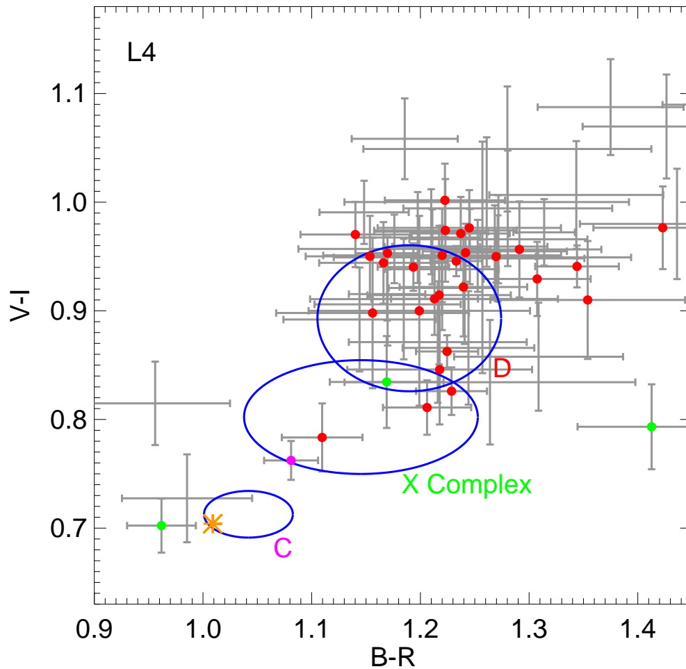
Figure 2.8: The taxonomic classifications for the brightest L4 Greeks are shown here at their mean color values. Red data points correspond to redder, D-type objects, green correspond to X-type and magenta correspond to C-type classifications as defined by Neese (2010) and Hasselmann et al. (2011). Ellipses designate the 1\sigma definitions for Bus-DeMeo taxonomies converted into BVRI colors. The yellow asterisk shows the position of solar colors (Ramírez et al. 2012), or the equivalent of a flat asteroid spectrum.
