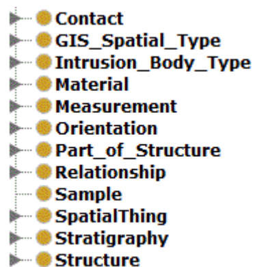
Figure 4.1 Screenshot showing the Top-Level Classes within the Geological Mapping Ontology
