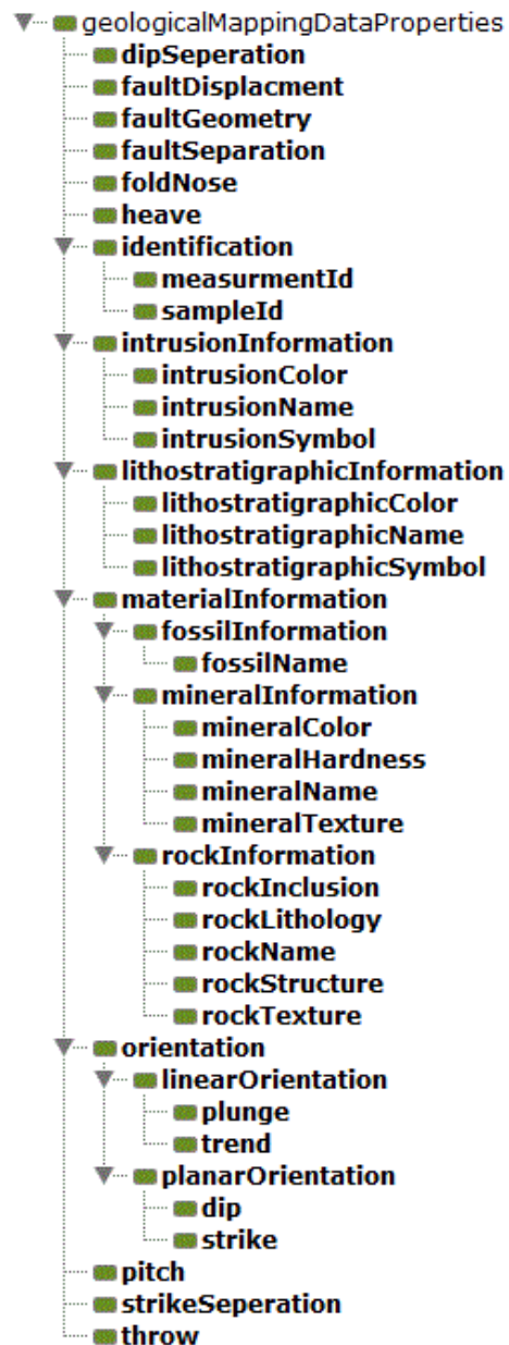
Figure 4.11 Screenshot of all the Data Properties within the Geological Mapping Ontology
