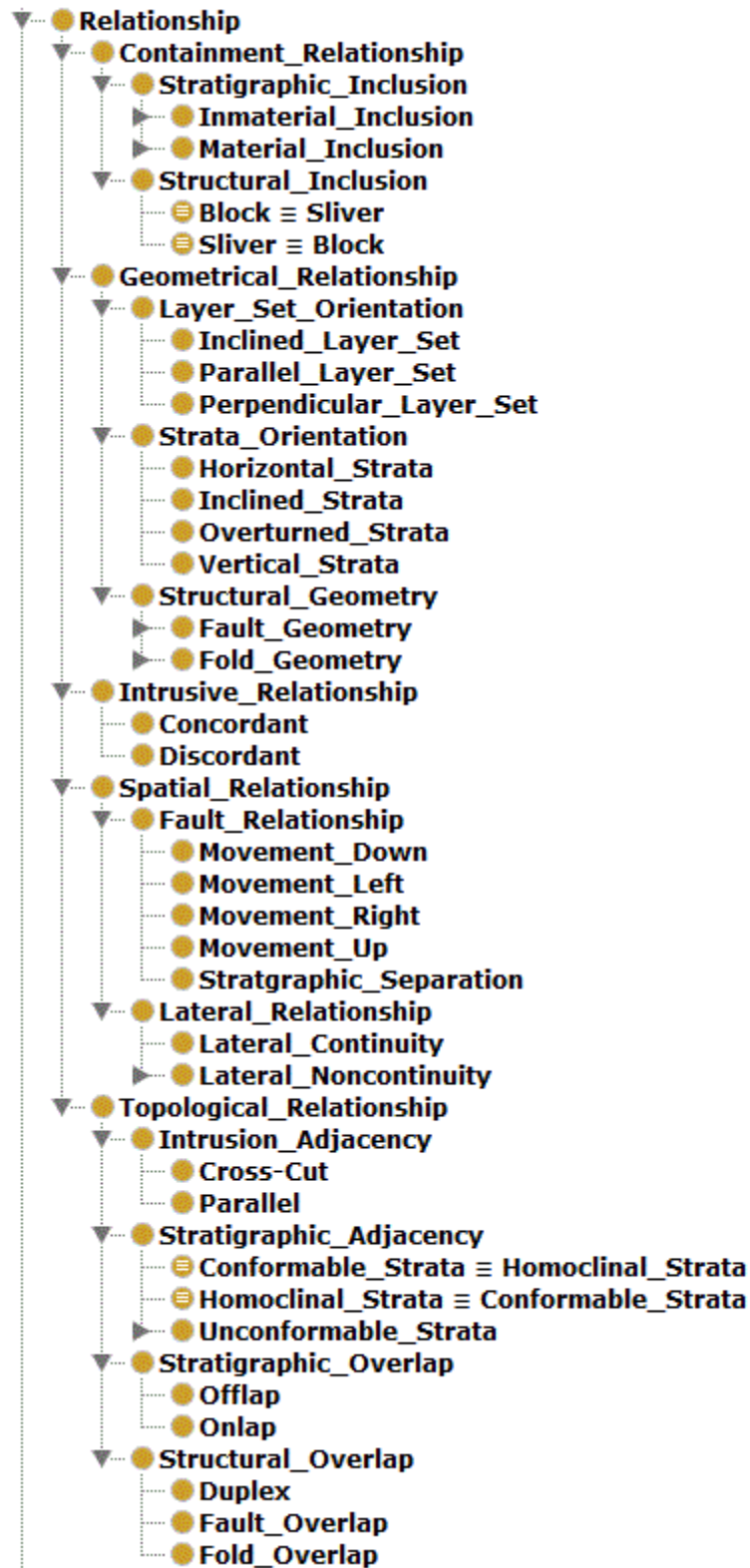
Figure 4.10 Screenshot of the Top-Level Class 'Relationship' up to three levels of Subclasses
