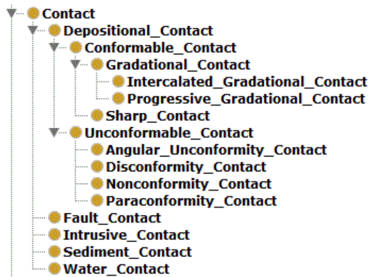
Figure 4.2 Screenshot of the Top-Level Class 'Contact' and all Subclasses
