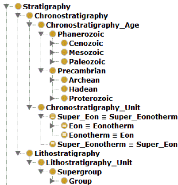
Figure 4.6 Screenshot of the Top-Level Class 'Stratigraphy' with both Subclasses 'Chronostratigraphy' and 'Lithostratigraphy' up to three levels of Subclasses
