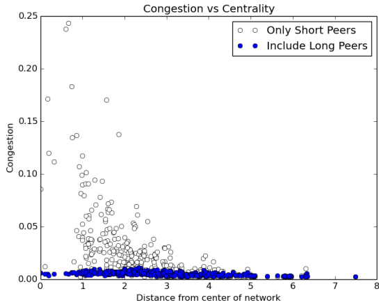
Figure 6.6: Here we see the congestion when using short peers only (approximating a scale free graph) and when utilizing randomly selected long peers. Using only short peers shows that central nodes handle disproportionate amounts of messages.
