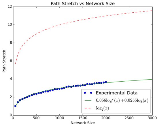
Figure 6.4: This data shows the experimental data points along with best fit curve and \log_2(x) curve as comparison.
