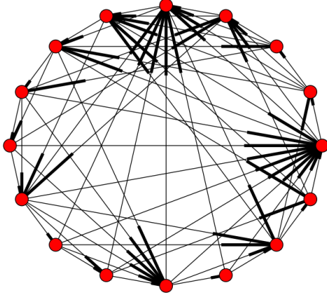
Figure 1.1: A Chord ring 16 nodes where m = 4 . The bold lines are incoming edges. Each node has a connection to its successor, as well as 4 fingers, some of which are duplicates.
