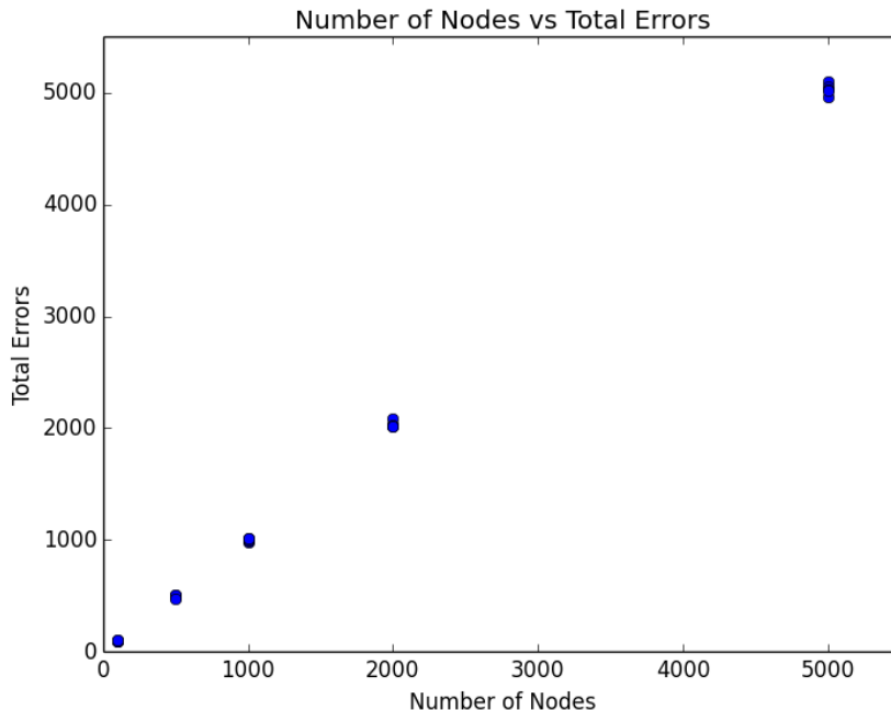
Figure 3.6: As the size of the graph increases, we see approximately 1 error per node.
