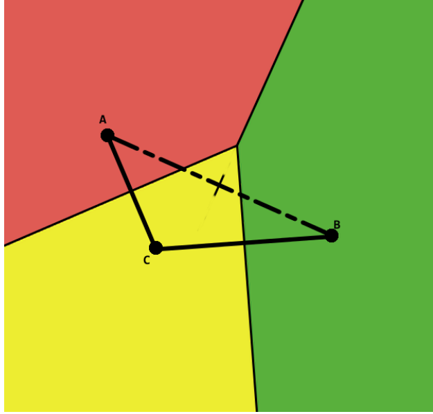
Figure 3.3: The edge between A and B is not detected by DGVH, as node C is closer to the midpoint than B is. This is mitigated by peer management polices.
