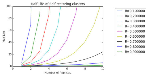
Figure 5.2: This graph shows the expected half-life of active clusters of replicas in response to churn. Note that the value for R dramatically effects behavior.
