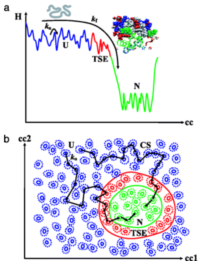
(Figure 1.1: A schematic description of protein folding. 'Frauenfelder')
