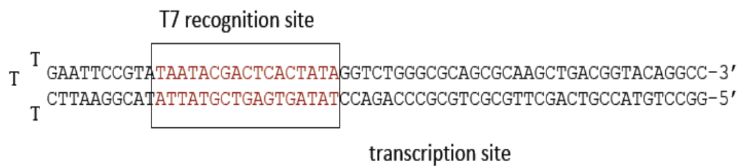
Figure 7 5'-3' RREIIB-Tr-DNA template is used in the RNA transcription reaction to synthesize RREIIB-Tr-RNA by purified T7 RNA polymerase.
