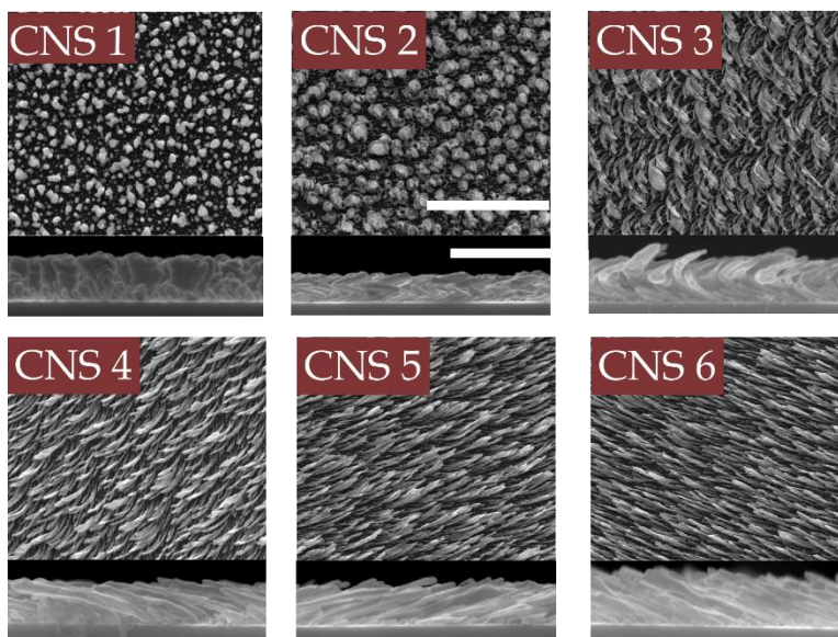
Figure 2.1 Scanning electron microscope images of Ag:Ti composite chiral nanorod structures CNS 1 to 6. In each of the six images, the upper portion represents the top view and the lower portion, the cross sectional side view of the samples. The scale bars in the top and side views are 2 \mu\text{m} and 500 nm.
