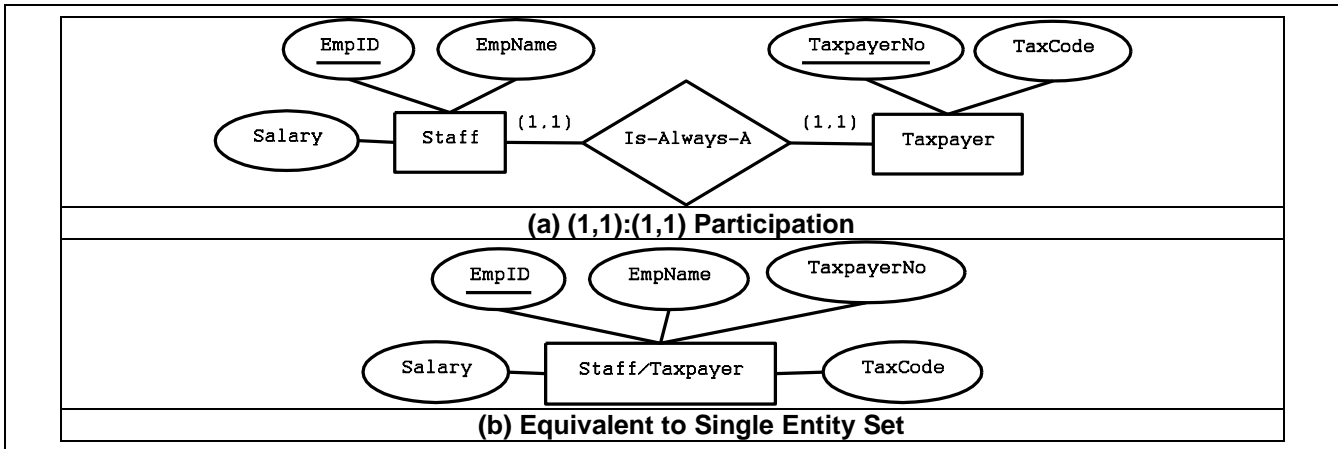
Figure 6. Equivalencies Between (1,1) Participation Relationship Sets
