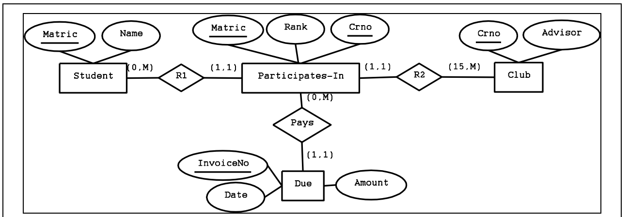
Figure 4. Syntactically Correct Way of Linking Due to Participates-in
