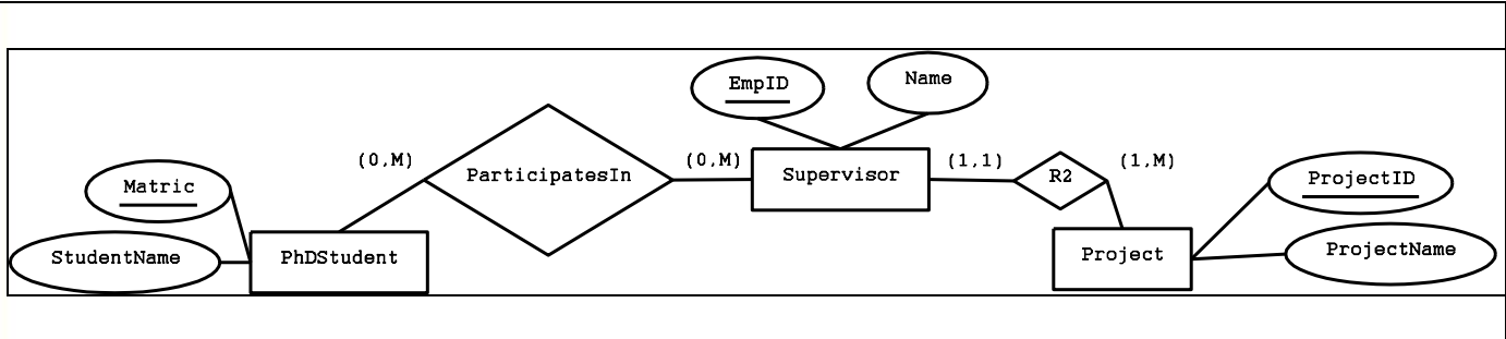
Figure 21. Structurally Representative E-R Diagram of BCNF
