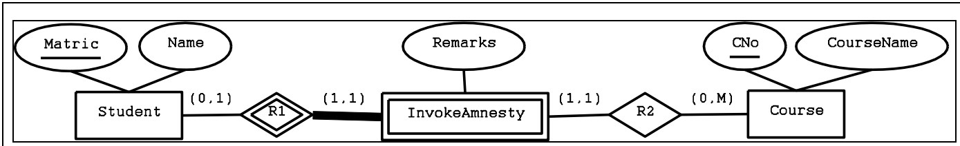
Figure 14. (0,1):(0,M) Transformation of Student Invokes Amnesty for Course
