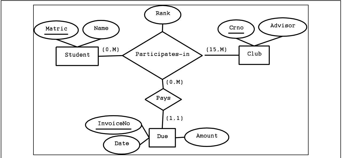
Figure 3. Syntactically Incorrect Way of Linking Due to Participates-in
