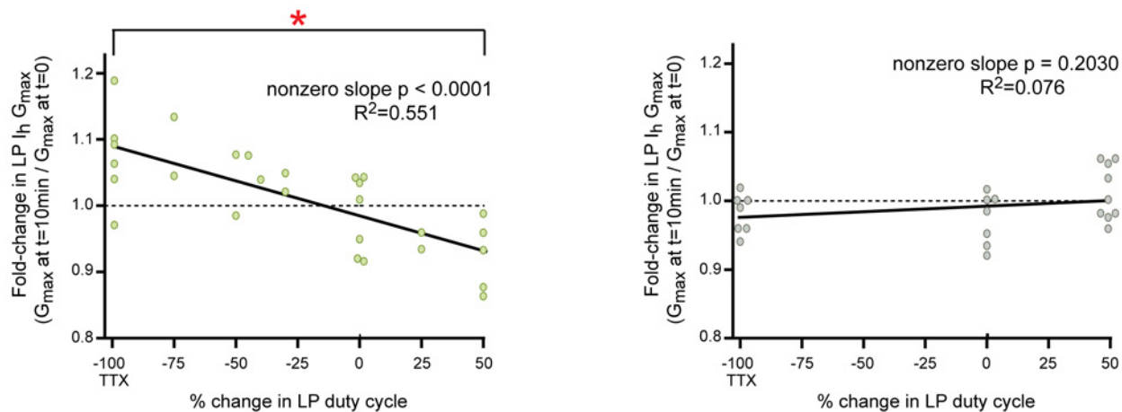
Fig 3. Tonic 5nM DA endows LP I h with activity dependence. (A) Experimental protocol. Activity was recorded with extracellular electrodes throughout the experiment. Measures of activity were obtained at t = -10min. The diagram shows how these measures were used in conjunction with TEVC to create a recurring voltage step that mimicked slow oscillatory activity at t = -10min. A change in LP burst duration was created by varying the length of the depolarizing step, as shown. Note that cycle period was maintained regardless of the change in burst duration; i.e., a change in burst duration was accompanied by a corresponding change in interburst duration. Duty cycle is defined as burst duration/cycle period; thus, our manipulations altered burst duration and duty cycle to the same extent. At t = -5min TTX was added to the superfusate. At t = 0, LP I h was measured with TEVC (black asterisk). Afterward, from t = 0 to 10min, 5nM DA was (B) or was not (C) added to the superfusate and TEVC was used to either hold the cell at its initial membrane potential in TTX (-100), or implement a recurrent voltage step (-75 to +50). At t = 10min, LP I h was again measured with TEVC (black asterisk). The experiment terminated at this point and a single preparation was not used further for additional experiments. (B-C) LP I h activity dependence curves. For every experiment in 5nM DA (B) or saline (C), the fold-change in LP I h G max at t = 10min (i.e. G max at t = 10 ÷ G max at t = 0) was plotted against the % change in LP duty cycle and a linear regression was used to fit the data. Each data point on the plots represents one experiment and 51 animals were used to obtain the data shown in the plots; -100 on the x-axis represents experiments in TTX without a recurring step, i.e., complete activity blockade. Each line represents a linear regression analysis and the resulting R 2 and p values are shown on the graph. Red asterisk indicates that LP I h G max was significantly different at -100 and +50 in the presence but not absence of 5nM DA as determined using one-way ANOVAs with Tukey's multiple comparisons post hoc tests to analyze the -100, 0, and +50 groups (5nM DA: F(2,17) = 8.464; p = 0.0035; saline: F(2,22) = 2.326; p = 0.1236).
