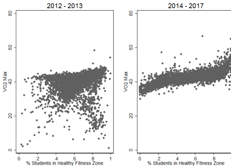
Figure A.17: Data Issues in Aerobic Capacity
