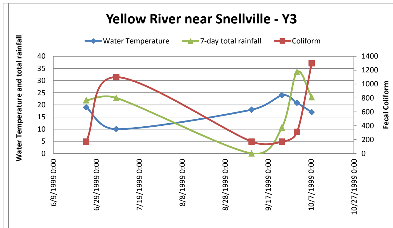
Figure 74. Relationship of fecal coliform, water temperature and the total rainfall 7 days prior to the water quality reading for the Yellow River station 3 near Snellville, Georgia for after June 17, 1999.
