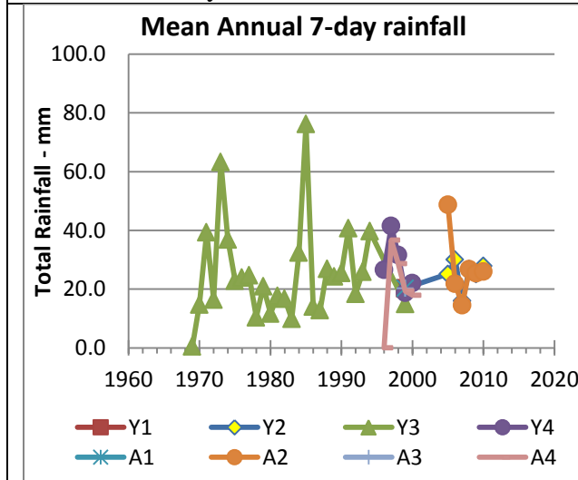
Figure 69. Annual mean 7-day total rainfall for the Yellow and Alcovy River basins in Gwinnett County, GA.
