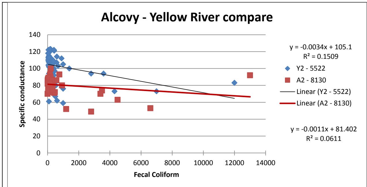
Figure 45. Scatter plot of fecal coliform with specific conductance with linear regression lines for the Yellow River basin Station Y2 and the Alcovy River basin station A2.
