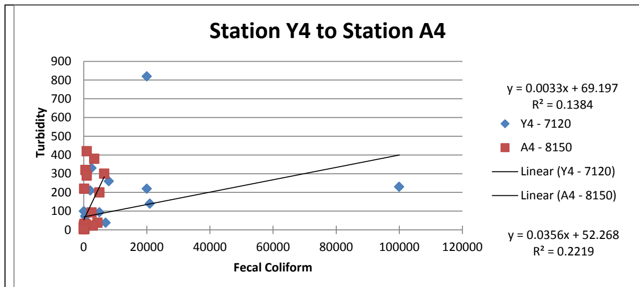
Figure 29. Relationship of Turbidity to fecal coliform at the Yellow River Station 4 and the Alcovy River station 4.
