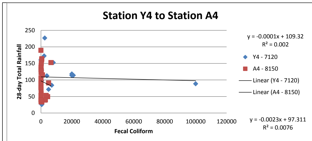
Figure 41. The relationship between the amount of rainfall 28 days prior to the water quality measurement and fecal coliform.
