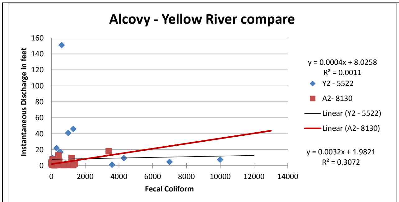
Figure 50. Scatter plot of fecal coliform with instantaneous discharge in feet with linear regression lines for the Yellow River basin Station Y2 and the Alcovy River basin station A2.
