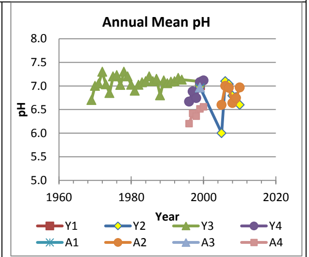
Figure 66. Annual mean pH for the Yellow and Alcovy River basins in Gwinnett County, GA.
