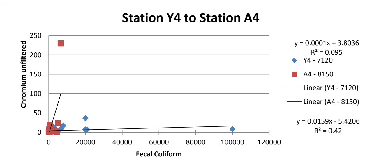
Figure 16. Relationship of Chromium to fecal coliform at the Yellow River Station 4 and the Alcovy River station 4.
