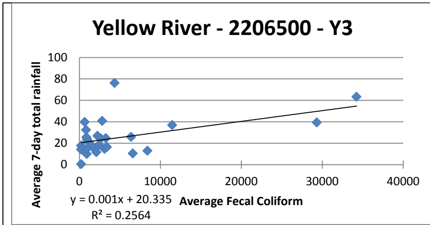
Figure B5. Yellow River Station 3 Annual Average 7 day Total Rainfall to Fecal Coliform Scatter plot with Least-squared linear regression line.
