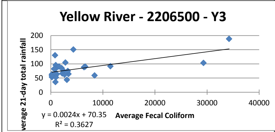
Figure B7. Yellow River Station 3 Annual Average 21 day Total Rainfall to Fecal Coliform Scatter plot with Least-squared linear regression line.
