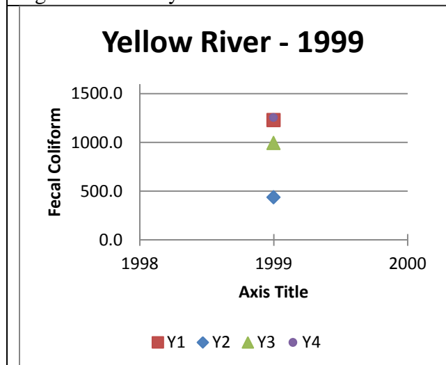
Figure 62. Mean fecal coliform values for the Yellow River basin in 1999.
