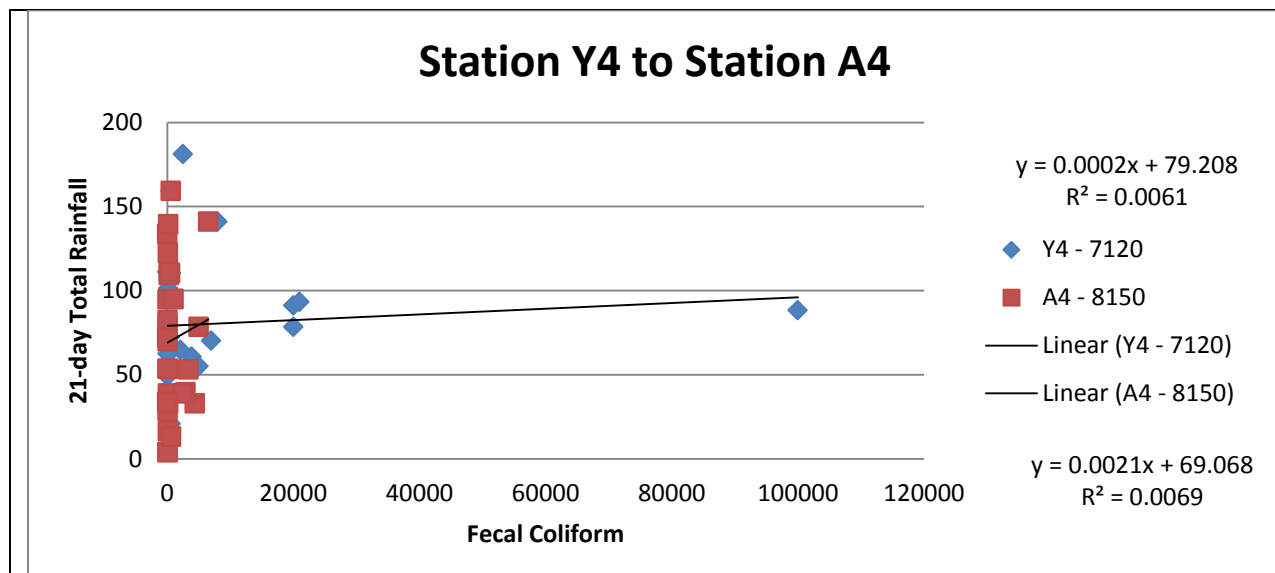
Figure 40. The relationship between the amount of rainfall 21 days prior to the water quality measurement and fecal coliform.
