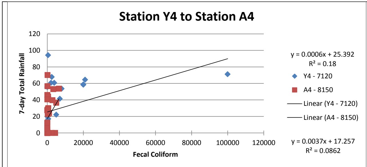
Figure 38. The relationship between the amount of rainfall 7 days prior to the water quality measurement and fecal coliform.
