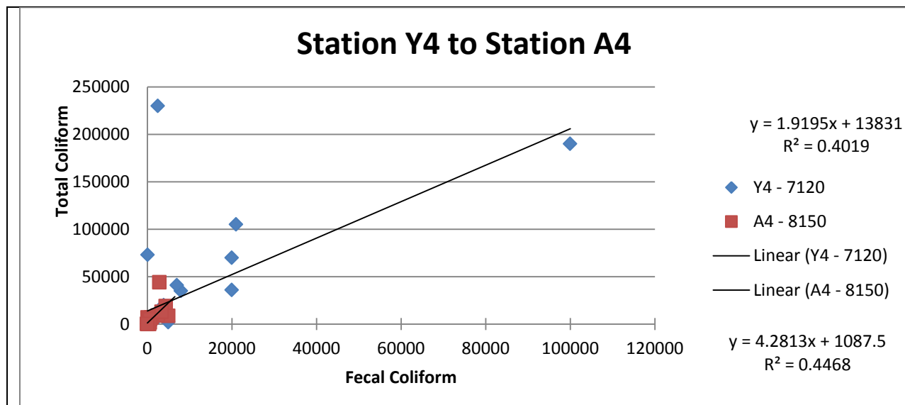
Figure 27. Relationship of Total Coliform to fecal coliform at the Yellow River Station 4 and the Alcovy River station 4.
