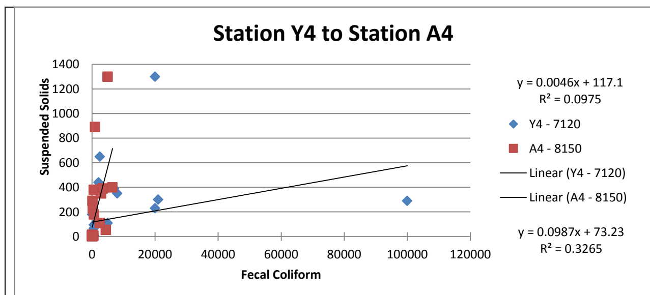
Figure 28. Relationship of Suspended Solids to fecal coliform at the Yellow River Station 4 and the Alcovy River station 4.
