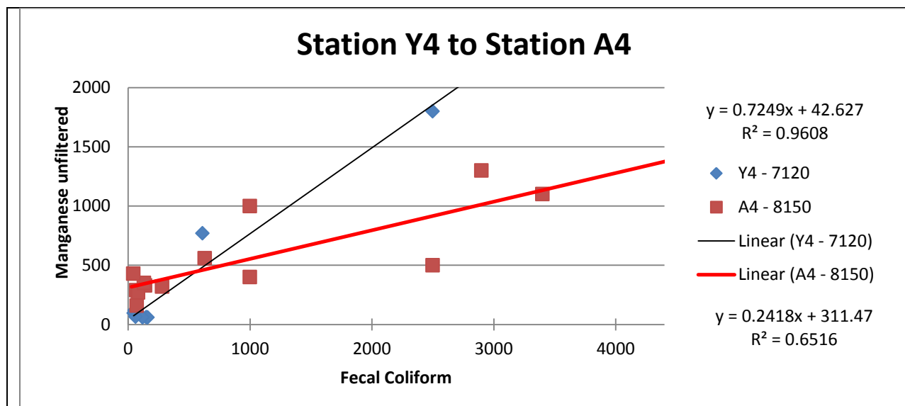
Figure 17. Relationship of Manganese to fecal coliform at the Yellow River Station 4 and the Alcovy River station 4.
