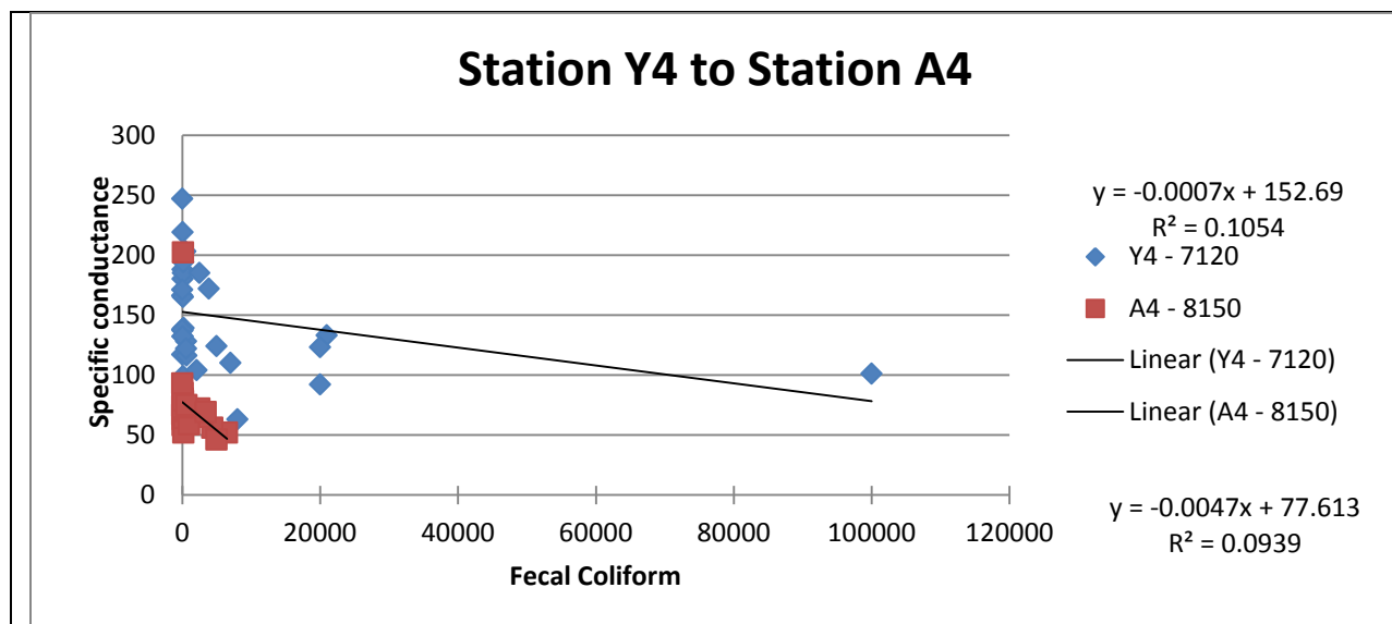
Figure 30. Relationship of Specific Conductance to fecal coliform at the Yellow River Station 4 and the Alcovy River station 4.
