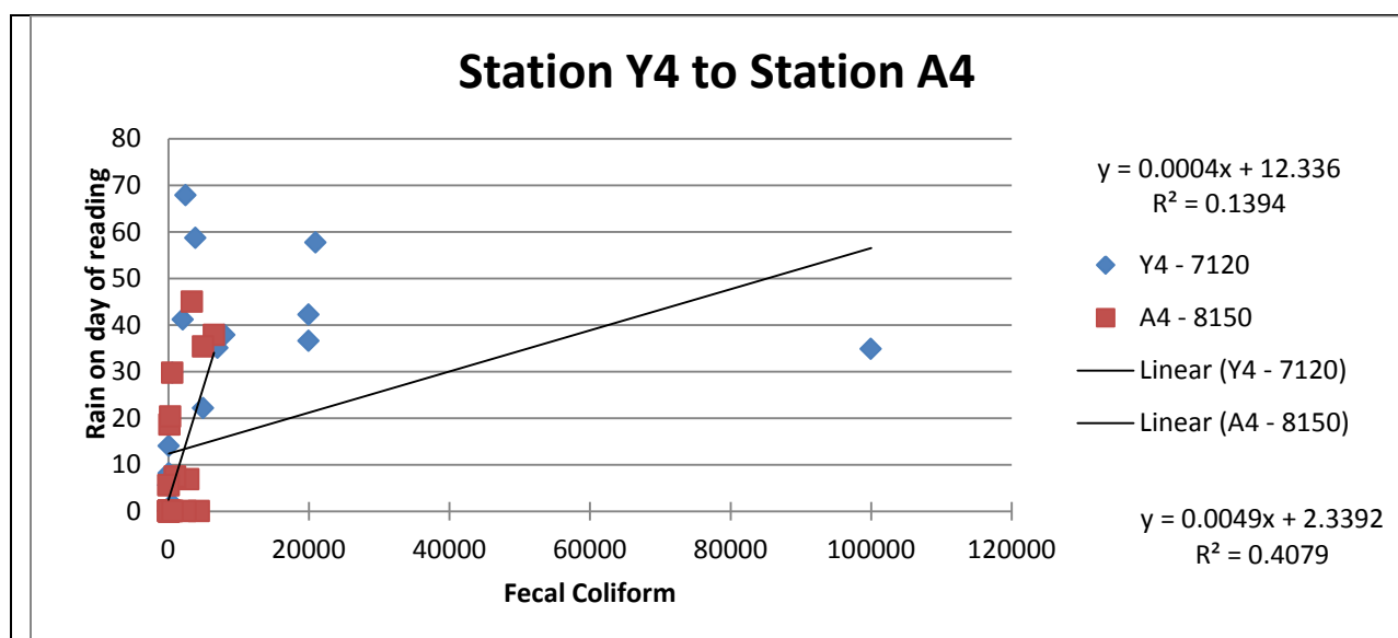
Figure 34. The relationship between fecal coliform and the amount of rain that occurs on the day the water quality reading was taken.
