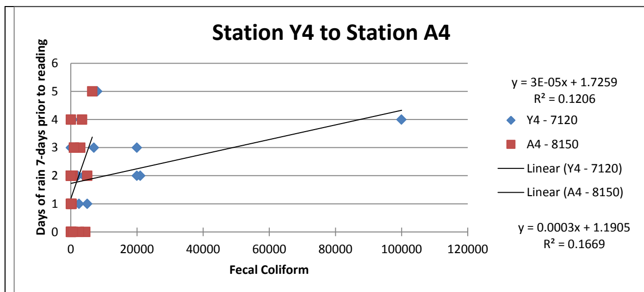
Figure 35. The relationship between fecal coliform and the number of days of rain 7 days prior to the water quality reading was taken.
