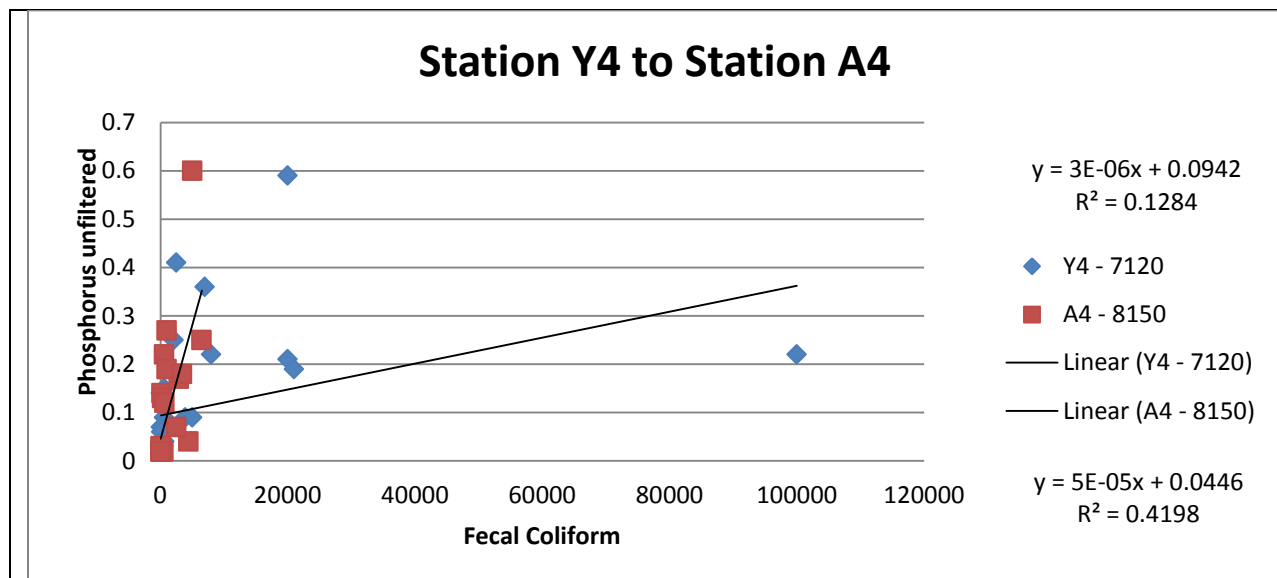
Figure 23. Relationship of Phosphorus to fecal coliform at the Yellow River Station 4 and the Alcovy River station 4.
