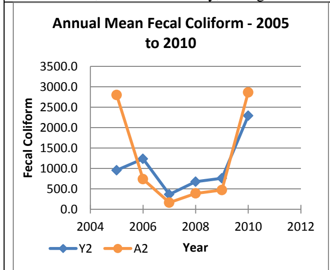
Figure 65. Annual mean fecal coliform for 2005 to 2010 for the Yellow River basin station 2 and the Alcovy River basin station 2.
