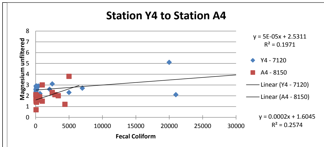
Figure 18. Relationship of Magnesium to fecal coliform at the Yellow River Station 4 and the Alcovy River station 4.
