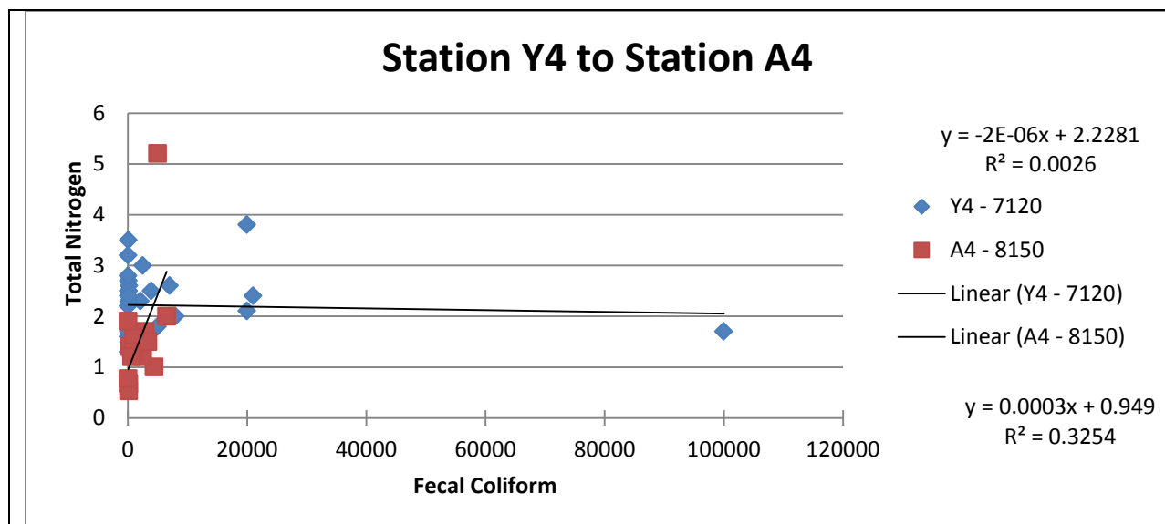
Figure 22. Relationship of Total Nitrogen to fecal coliform at the Yellow River Station 4 and the Alcovy River station 4.
