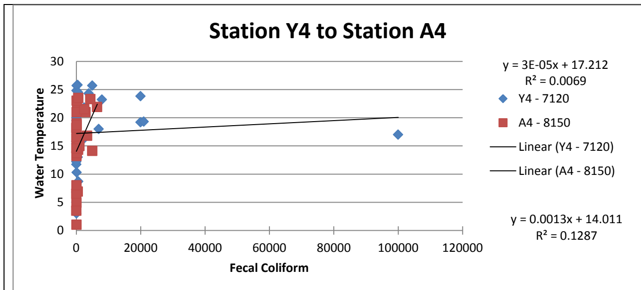
Figure 32. Relationship of Water Temperature to fecal coliform at the Yellow River Station 4 and the Alcovy River station 4.
