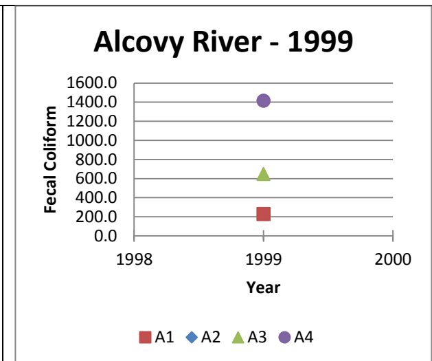
Figure 63. Mean fecal coliform values for the Alcovy River basin in 1999.
