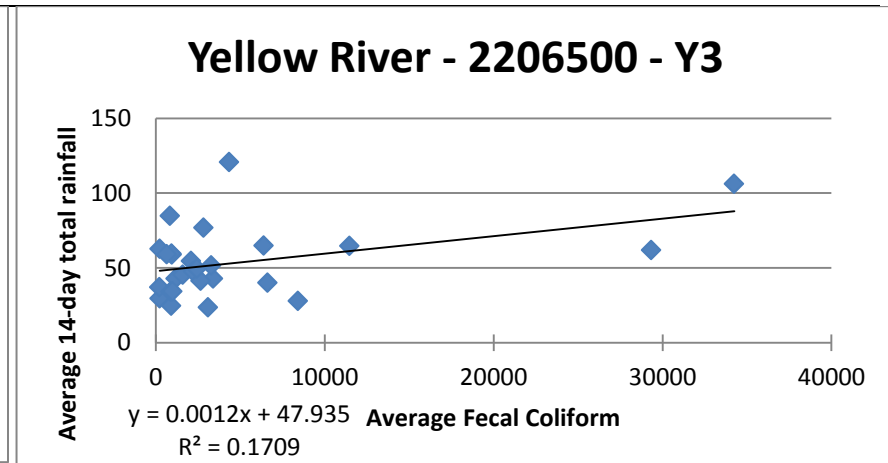
Figure B6. Yellow River Station 3 Annual Average 14 day Total Rainfall to Fecal Coliform Scatter plot with Least-squared linear regression line.
