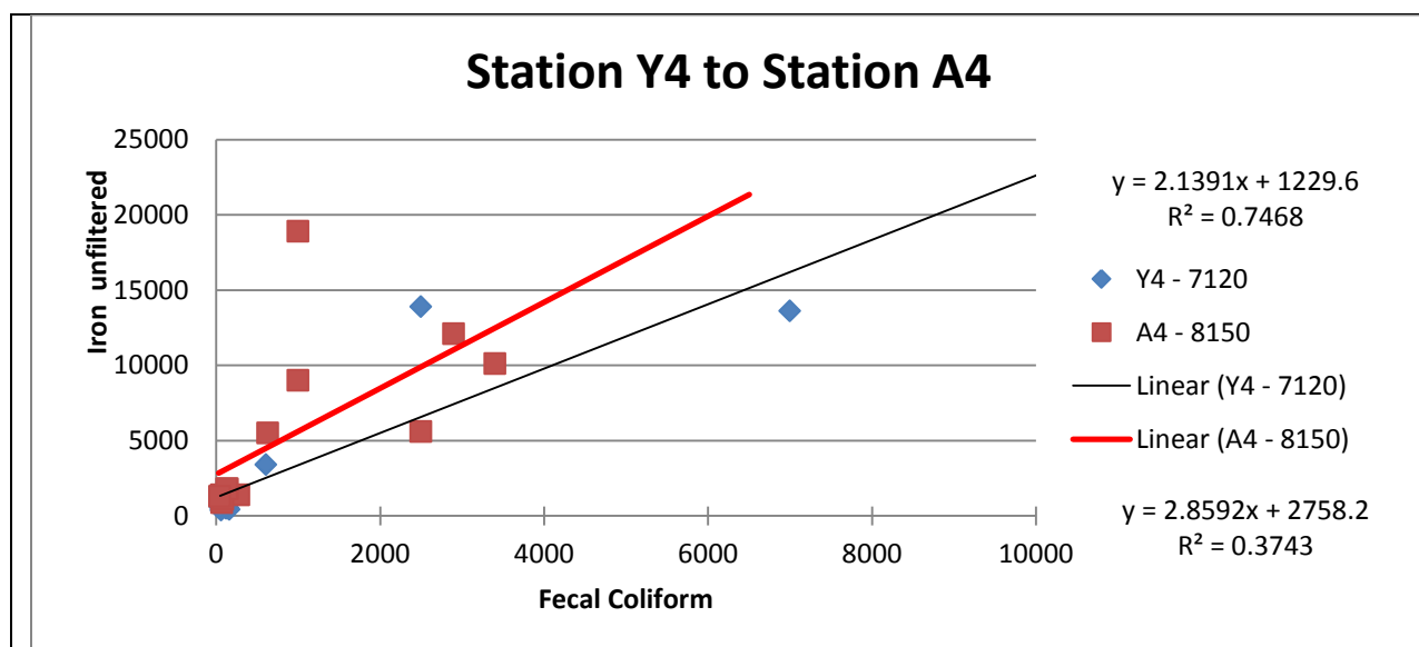
Figure 19. Relationship of Iron to fecal coliform at the Yellow River Station 4 and the Alcovy River station 4.
