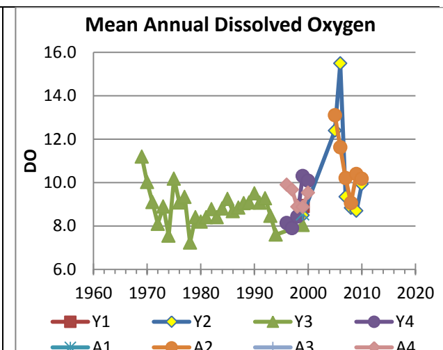
Figure 68. Annual mean dissolved oxygen for the Yellow and Alcovy River basins in Gwinnett County, GA.
