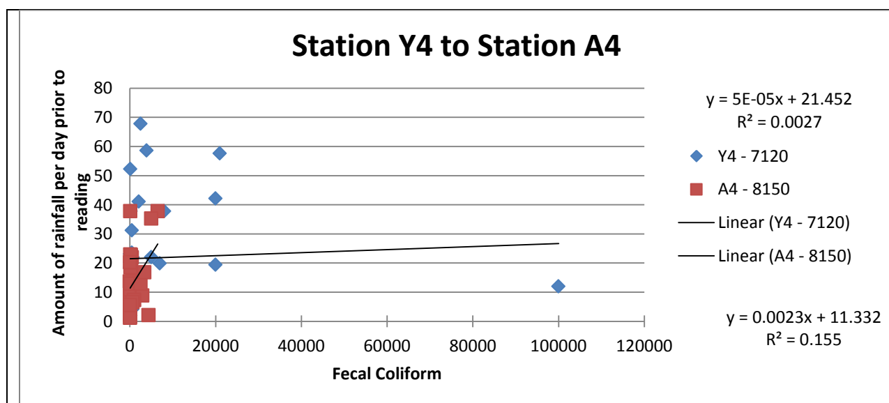
Figure 36. The relationship between fecal coliform and the amount of rainfall per day prior to the water quality reading.
