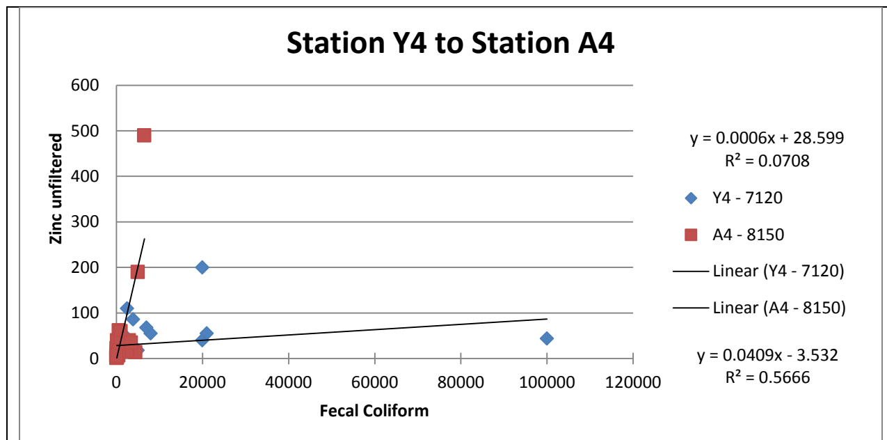
Figure 14. Relationship of Zinc to fecal coliform at the Yellow River Station 4 and the Alcovy River station 4.
