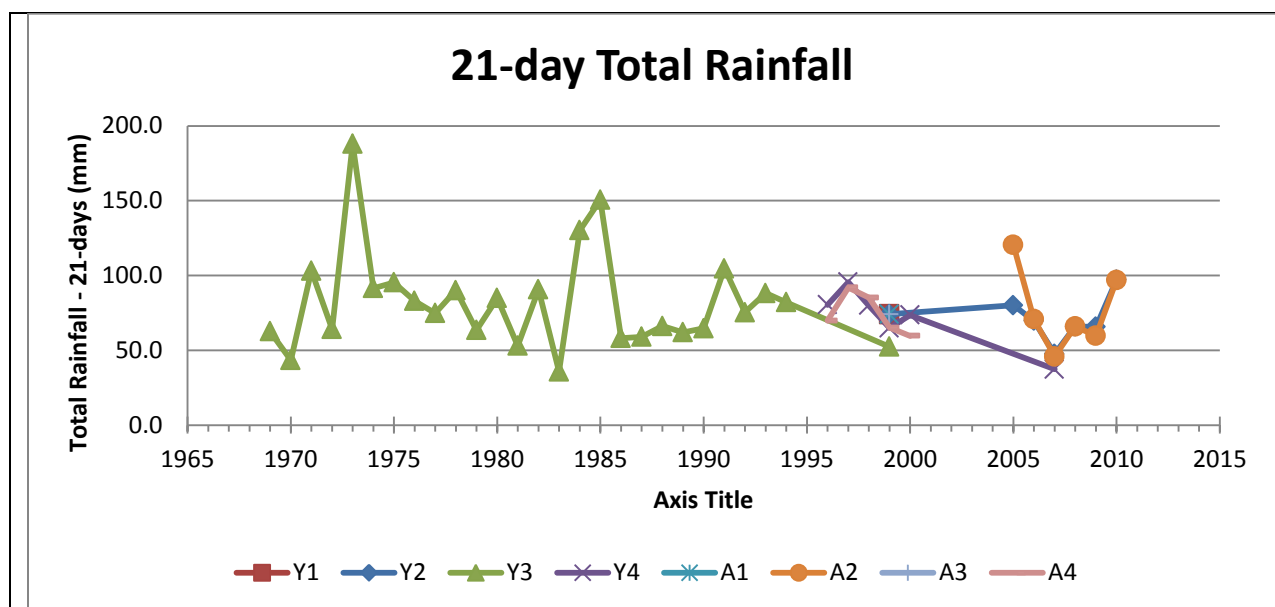
Figure 76. Mean Total Rainfall for the 21-day period prior to the water quality measurements for the Yellow and Alcovy River basins from 1969 to 2010.
