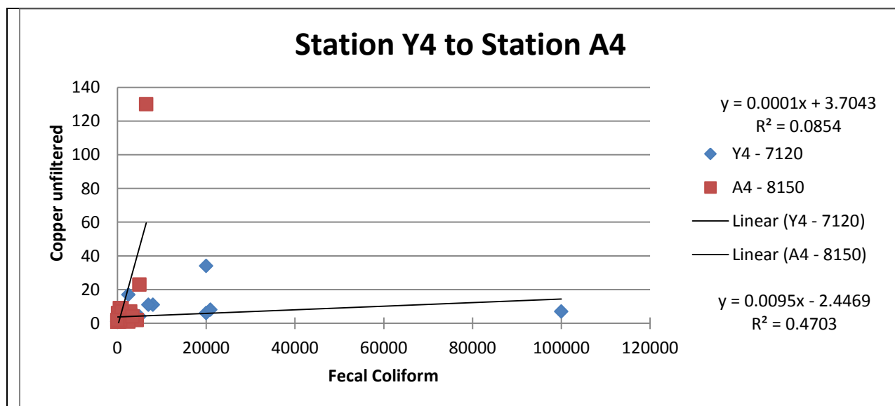
Figure 15. Relationship of Copper to fecal coliform at the Yellow River Station 4 and the Alcovy River station 4.
