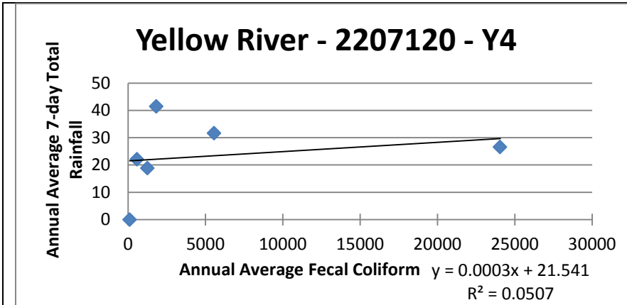
Figure B9. Yellow River Station 4 Annual Average 7 day Total Rainfall to Fecal Coliform Scatter plot with Least-squared linear regression line.
