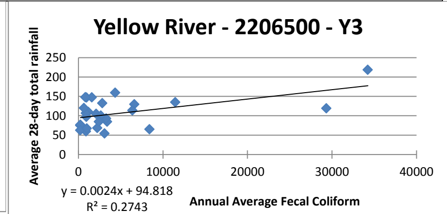
Figure B8. Yellow River Station 3 Annual Average 28 day Total Rainfall to Fecal Coliform Scatter plot with Least-squared linear regression line.
