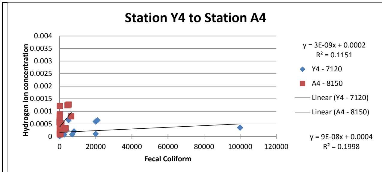
Figure 31. Relationship of Hydrogen Ion Concentration to fecal coliform at the Yellow River Station 4 and the Alcovy River station 4.
