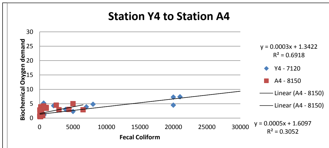
Figure 24. Relationship of Biochemical Oxygen Demand to fecal coliform at the Yellow River Station 4 and the Alcovy River station 4.
