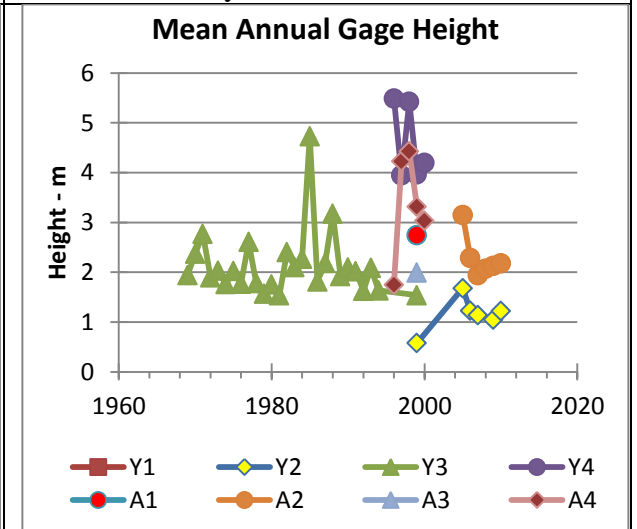
Figure 70. Annual mean Gage Height for the Yellow and Alcovy River basins in Gwinnett County, GA.
