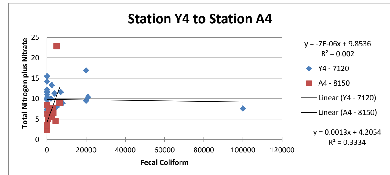
Figure 21. Relationship of Total Nitrogen plus nitrate to fecal coliform at the Yellow River Station 4 and the Alcovy River station 4.
