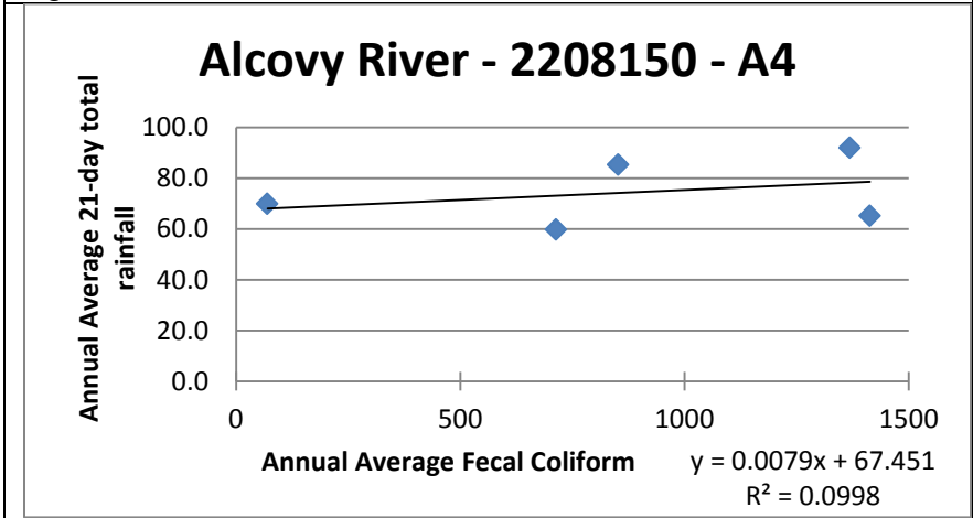
Figure B19. Alcovy River Station 4 Annual Average 21 day Total Rainfall to Fecal Coliform Scatter plot with Least-squared linear regression line.
