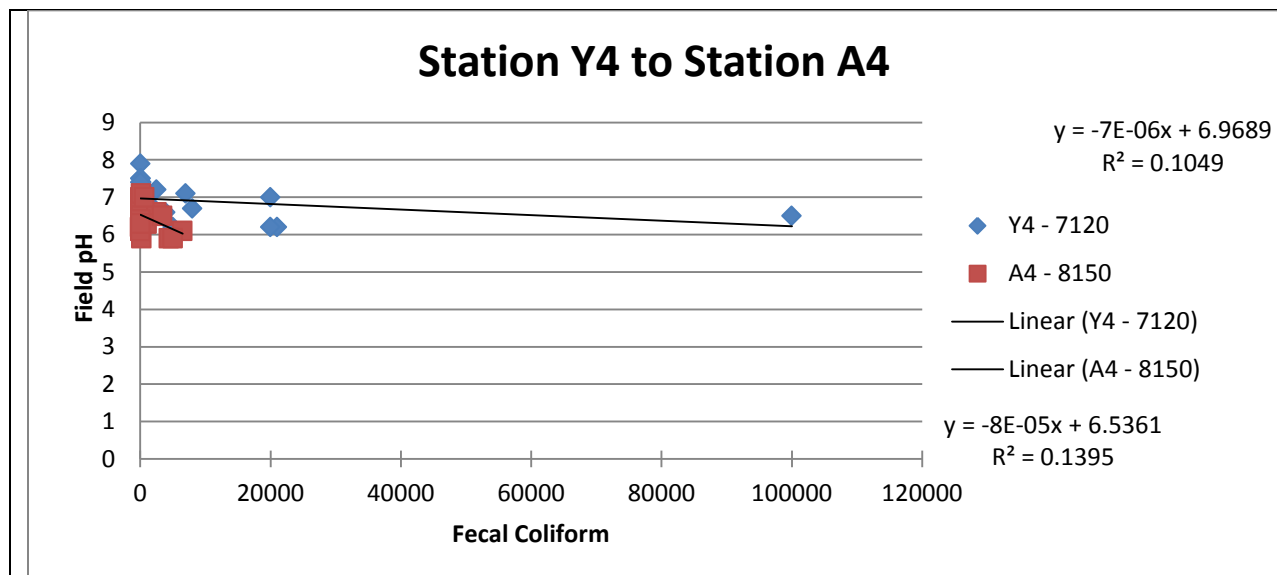
Figure 33. Relationship of pH (measured in the field) to fecal coliform at the Yellow River Station 4 and the Alcovy River station 4.
