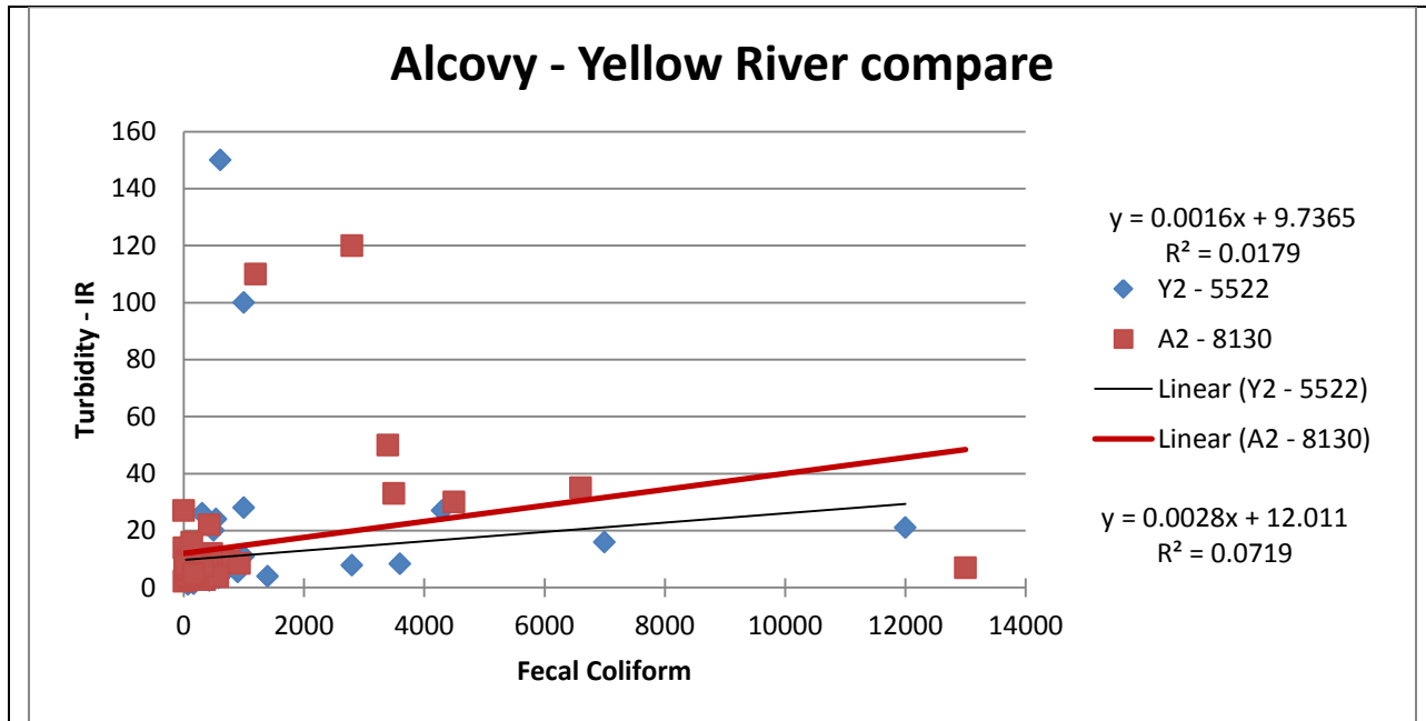
Figure 49. Scatter plot of fecal coliform with turbidity with linear regression lines for the Yellow River basin Station Y2 and the Alcovy River basin station A2.
