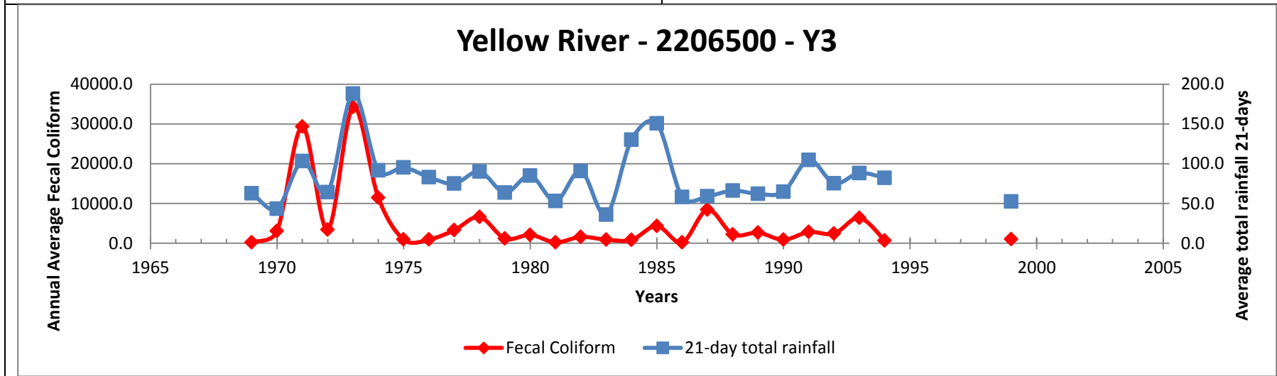
Figure 59. Mean Annual Fecal Coliform trend compared with Mean Annual 21 day total rainfall for the Yellow River basin station 3.
