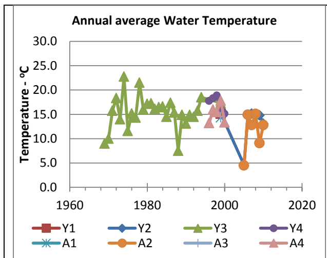
Figure 67. Annual mean water temperature for the Yellow and Alcovy River basins in Gwinnett County, GA.
