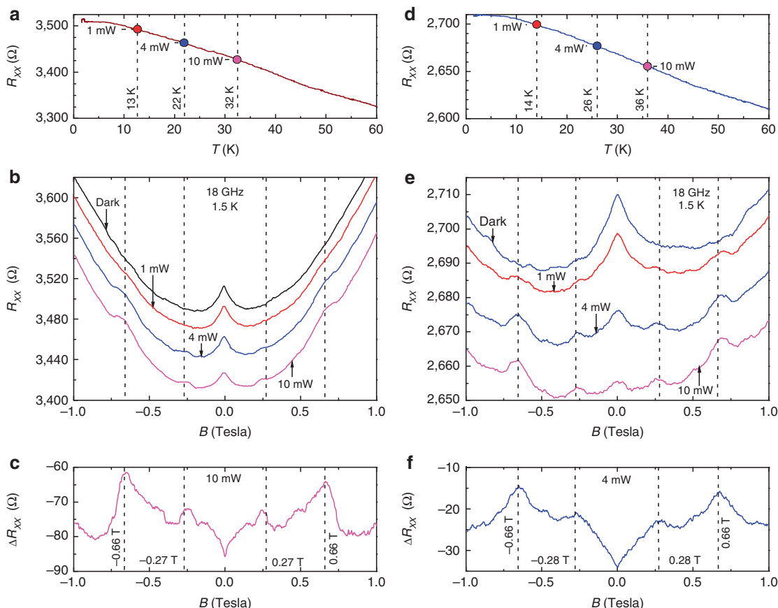
Figure 2 | Transport in single-layer graphene. Panels a–c show some results for sample 2, whereas d,f show representative data for sample 3. (a) Sample 2 shows a decrease in the resistance R_{xx} with increasing temperature T , that is, dR_{xx}/dT \leq 0 , in the absence of a magnetic field, that is, B = 0 T. (b) The data traces show a downward shift with increasing microwave power, P , at F = 18 GHz, suggestive of microwave-induced carrier heating in the specimen. The R_{xx} at B = 0 T obtained from these traces have been marked as filled circles in panel a above, which shows the T dependence of R_{xx} . Apparently, P = 10 mW serves to increase the carrier temperature up to T = 32 K in sample 2. Microwave-induced resonances appear in the vicinity of the dashed lines with increasing P . (c) \Delta R_{xx} = R_{xx}(10 \text{ mW}) - R_{xx}(\text{dark}) is shown versus the magnetic field for sample 2. Note the change in \Delta R_{xx} due to spin resonance in the vicinity of the dashed lines at B = \pm 0.66 and \pm 0.27 T. (d) Sample 3 also shows a decrease in the resistance R_{xx} with increasing temperature T , that is, dR_{xx}/dT \leq 0 , in the absence of a magnetic field, that is, B = 0 T. (e) At F = 18 GHz and T = 1.5 K, R_{xx} is shown versus B for sample 3, at several power levels. The R_{xx} at B = 0 T observed in these data have been marked as filled circles in panel d . (f) This panel shows \Delta R_{xx} = R_{xx}(10 \text{ mW}) - R_{xx}(\text{dark}) versus the magnetic field for sample 3. Note the change in \Delta R_{xx} due to spin resonance in the vicinity of B = \pm 0.66 and \pm 0.28 T.
